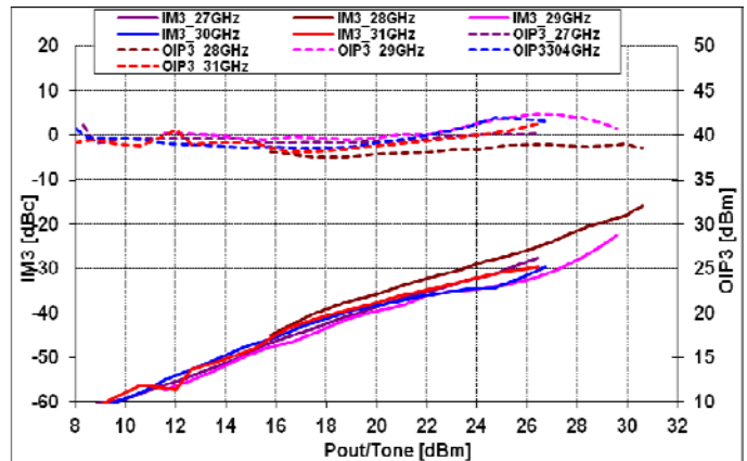
@Vds=5V, Idsq=1.5A
