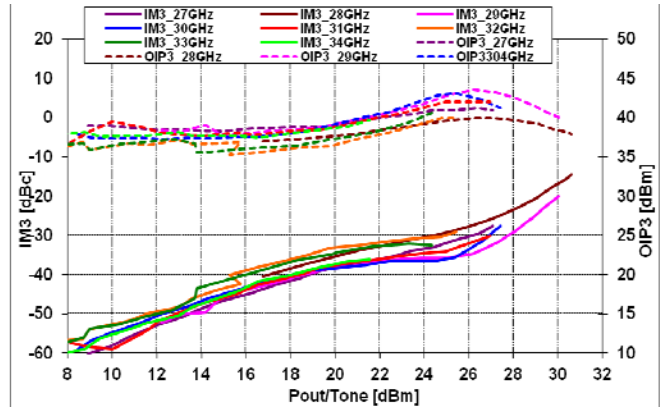
@Vds=5V, Idsq=2.6A
