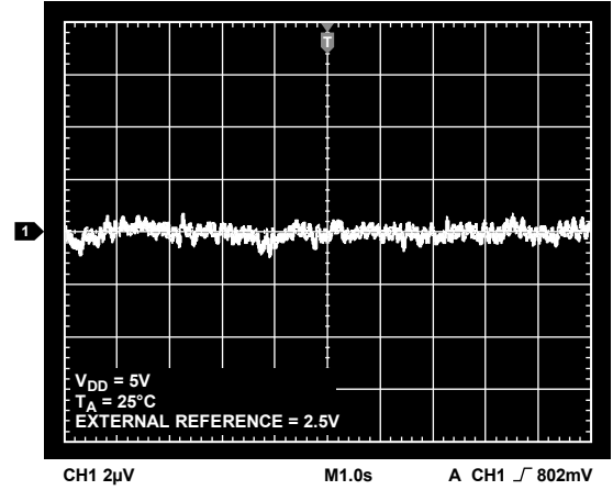
Figure 33. 0.1 Hz to 10 Hz Output Noise Plot, 2.5 V External Reference
