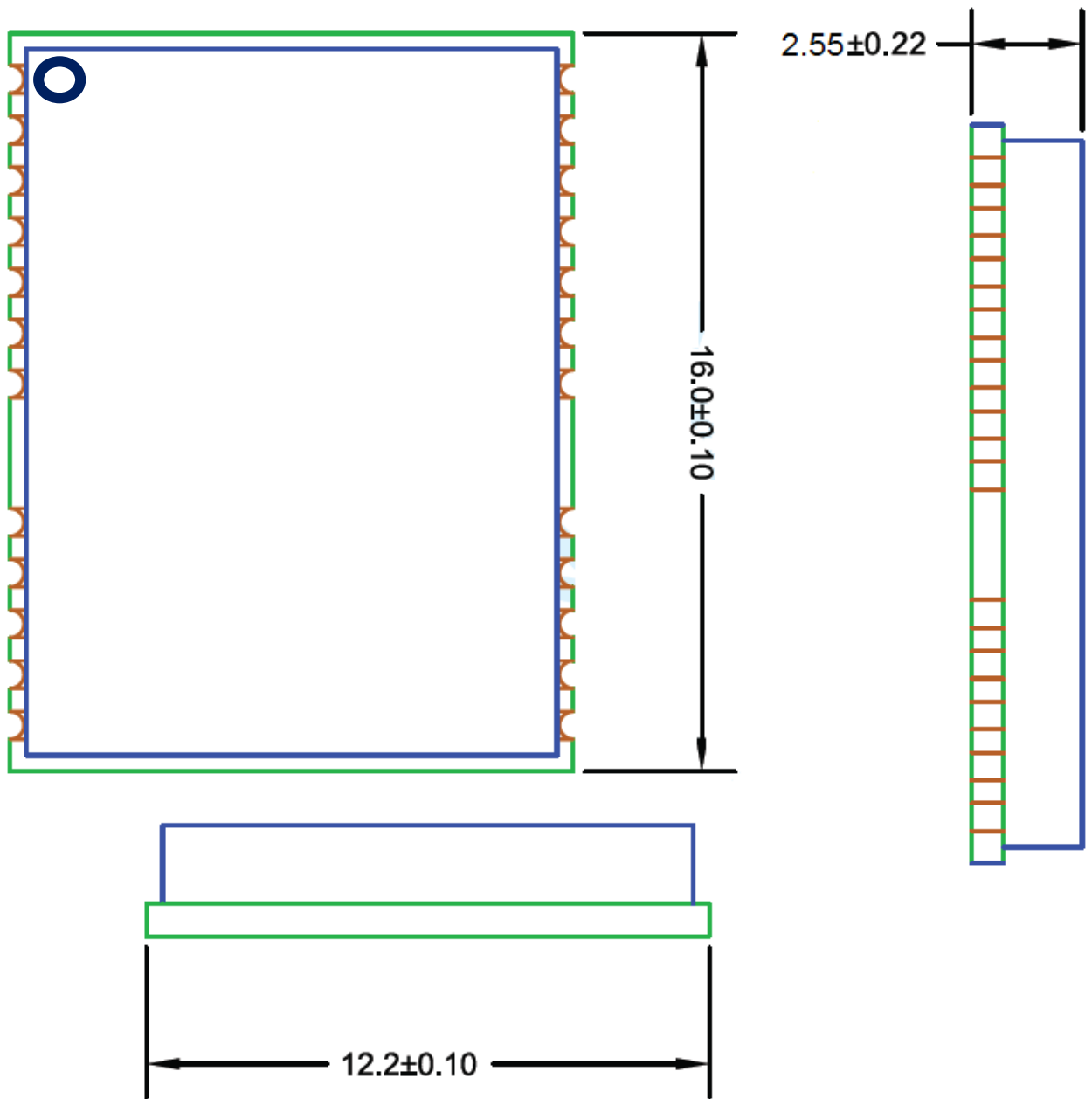
Figure 3 Package Outline Drawing (Top View) Dimensions are in mm
