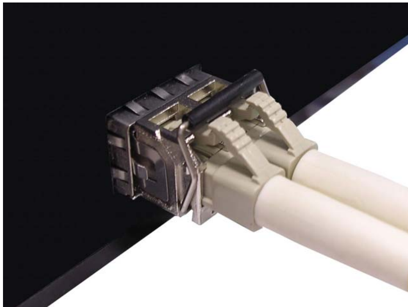
Figure 2.10: LC connected to the transceiver
