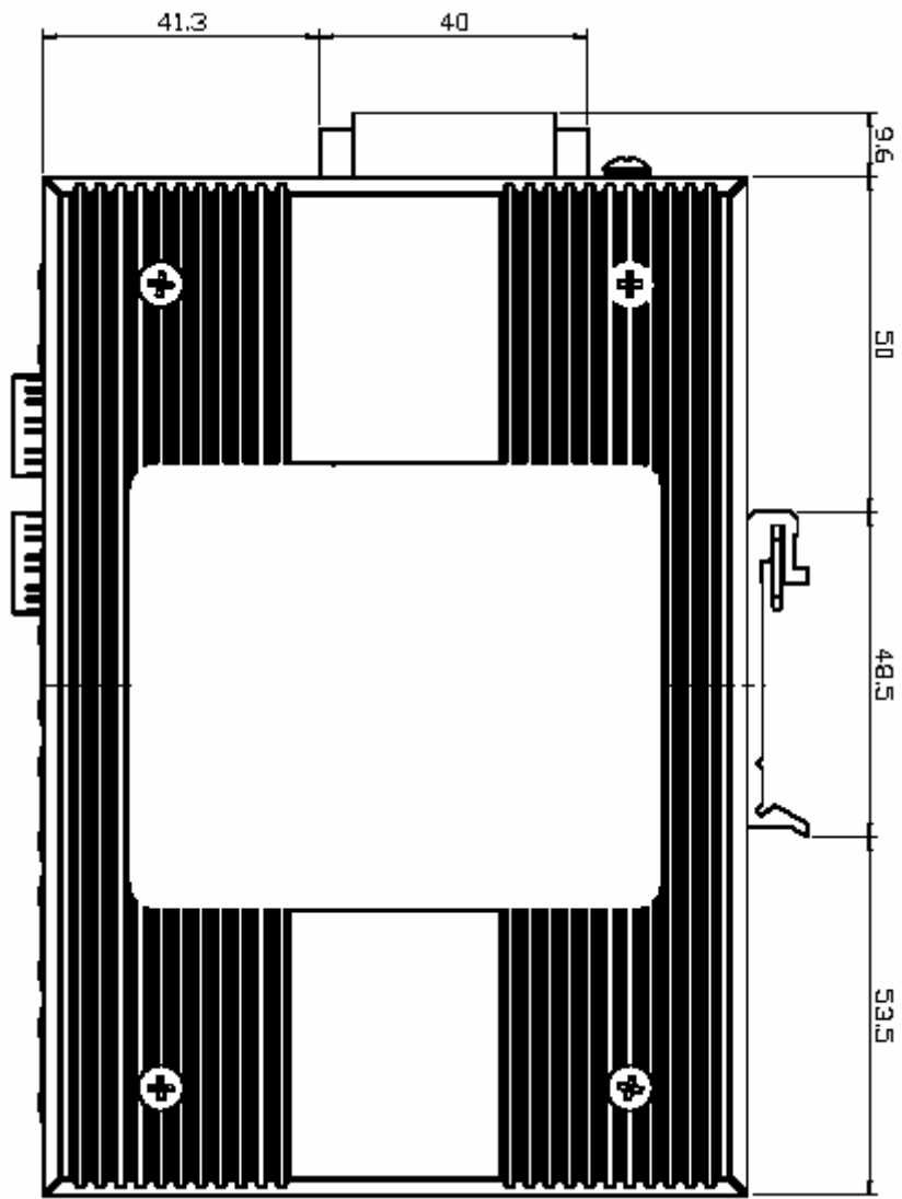
Figure 2.2: Side View
