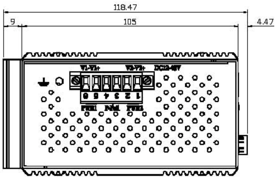
Figure 2.4: Top View
