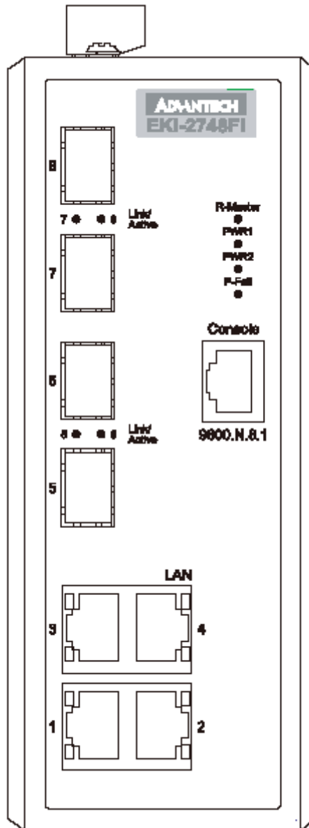
Figure 2.1: Front View
