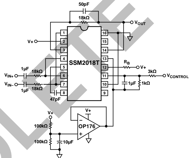
Figure 33. Single-Supply Operation of SSM2018
