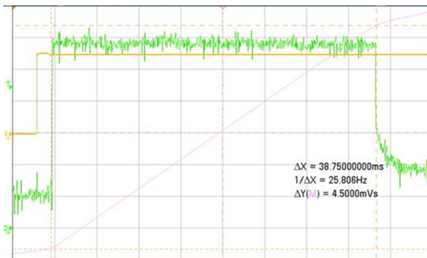
Inrush current of 4.5 mC with a duration of 38.7 mS
