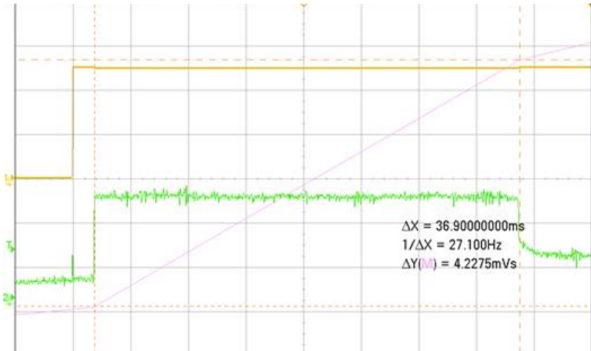
Inrush current of 4.22 mC with a duration of 36.9 mS
