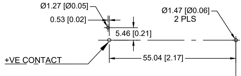
PCB LAYOUT
