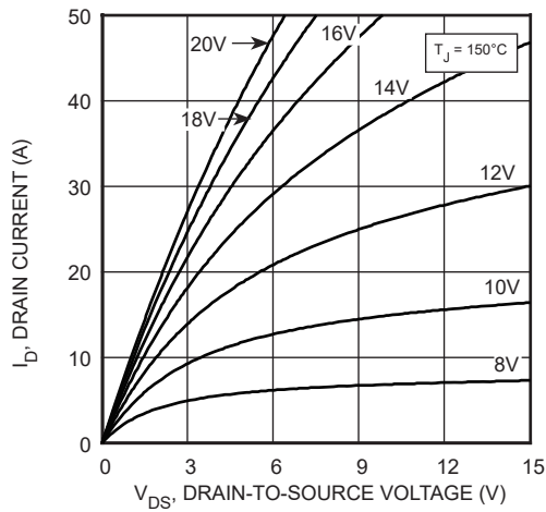
Figure 3, Output Characteristics
