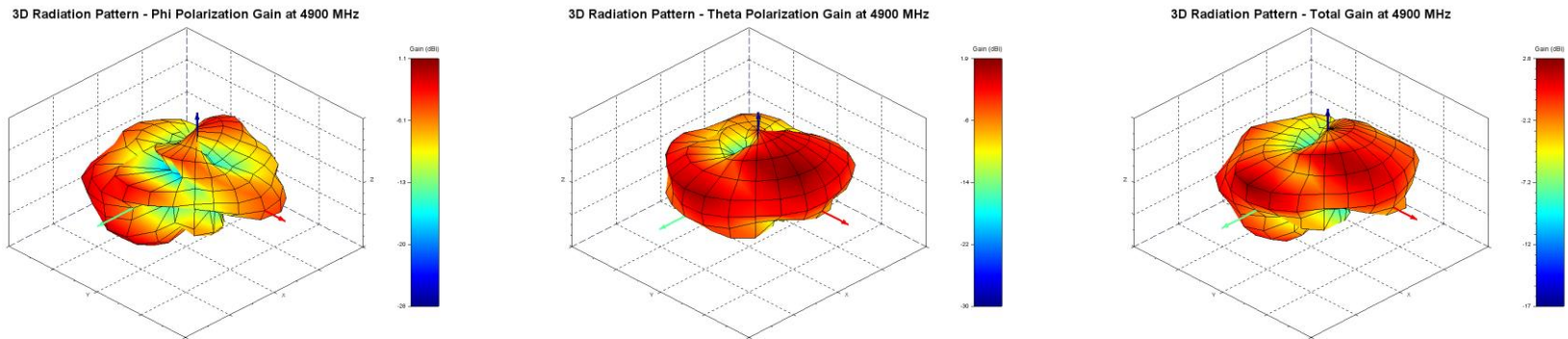
Figure 26 Phi, Theta, and Total Gain Plots
