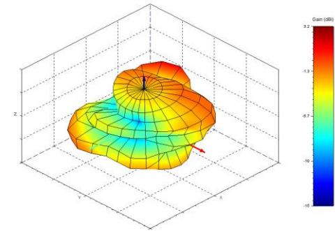
3D Radiation Pattern - Total Gain at 5400 MHz
