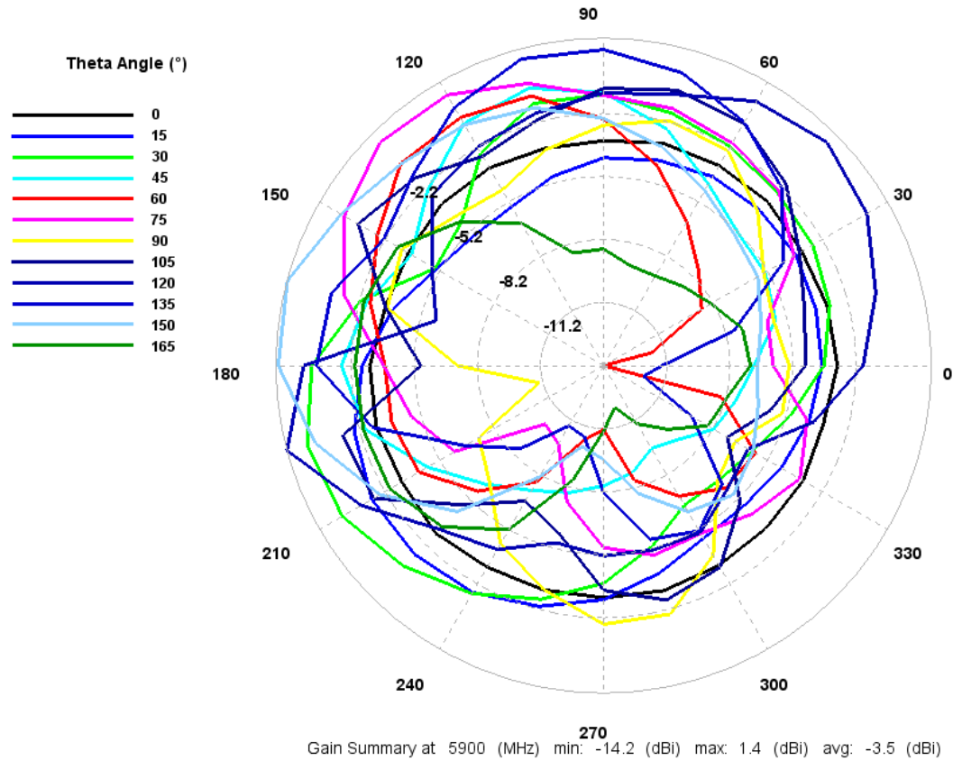
Azimuth Gain Pattern Cuts - Total Gain at 5900 MHz
