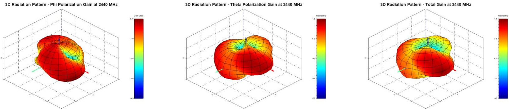
Figure 24 Phi, Theta, and Total Gain Plots
