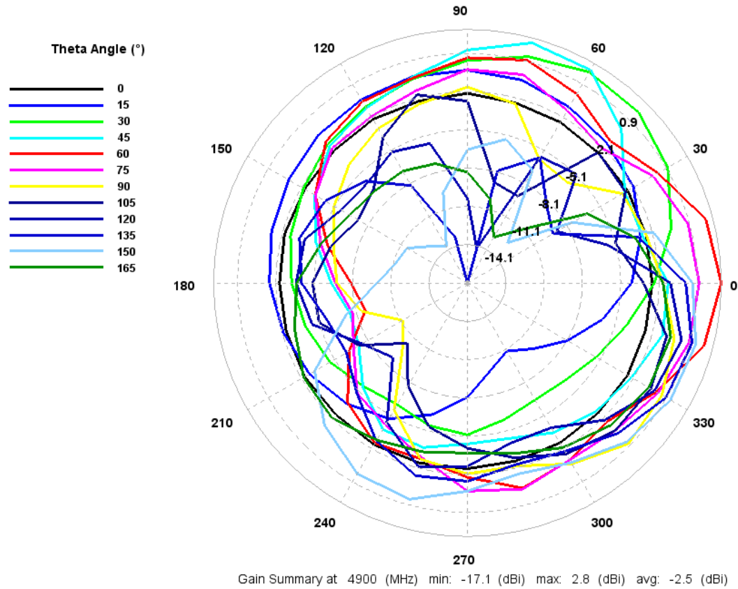
Azimuth Gain Pattern Cuts - Total Gain at 4900 MHz
