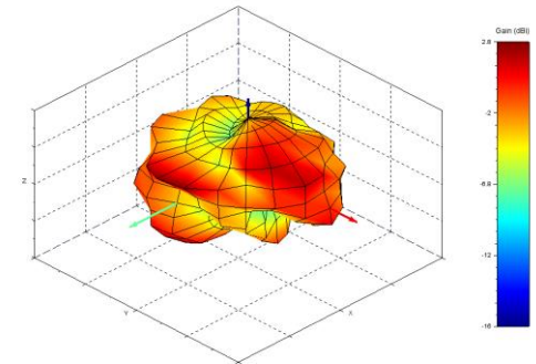
3D Radiation Pattern - Total Gain at 5400 MHz
