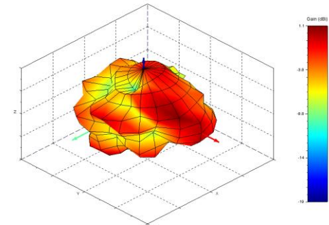
3D Radiation Pattern - Total Gain at 5900 MHz
