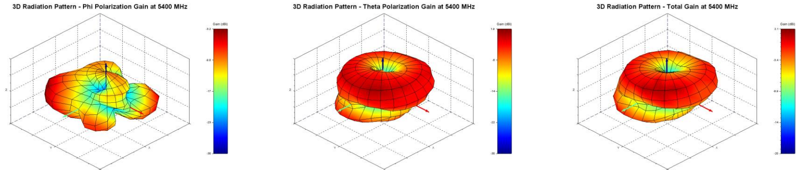
Figure 10 Phi, Theta, and Total Gain Plots
