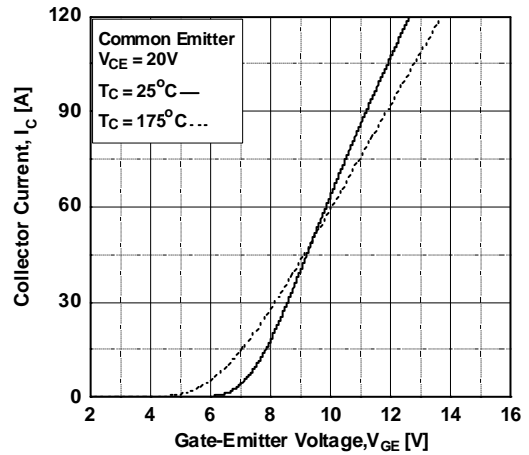
Figure 4. Transfer Characteristic
