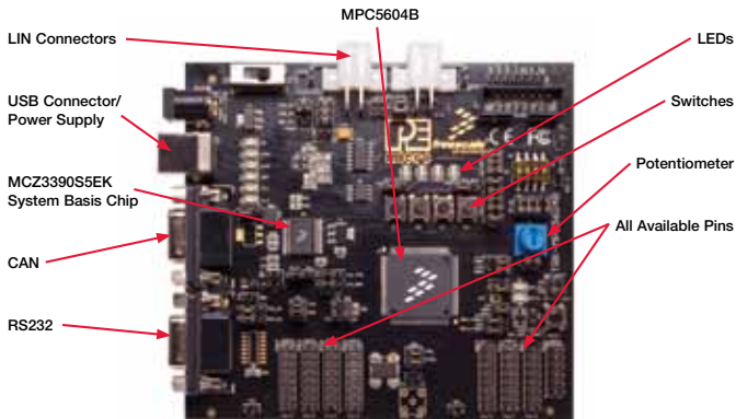
Figure 1: TRK-MPC5604B Board*
