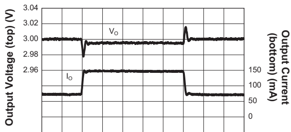
Load Transient Response LDO4 ( I_{OUT4} = 75mA to 150mA ; V_{BAT} = 3.6V ; V_{OUT4} = 3V ; C_{OUT} = 4.7\mu F )
