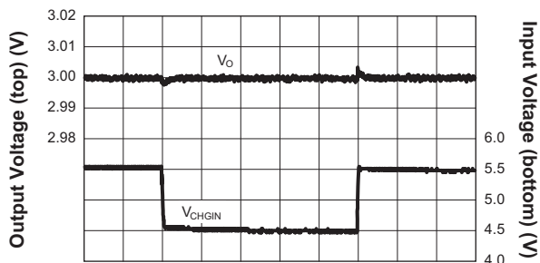
V_{CHGIN} Line Transient Response LDO4 ( V_{CHGIN} = 4.5V to 5.5V ; I_{OUT4} = 150mA ; V_{OUT4} = 3V )
