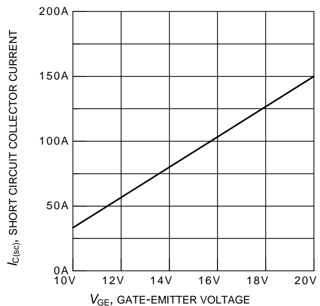
Figure 20. Typical short circuit collector current as a function of gate-emitter voltage ( V_{CE} \leq 600V , T_i = 150^\circ C )
