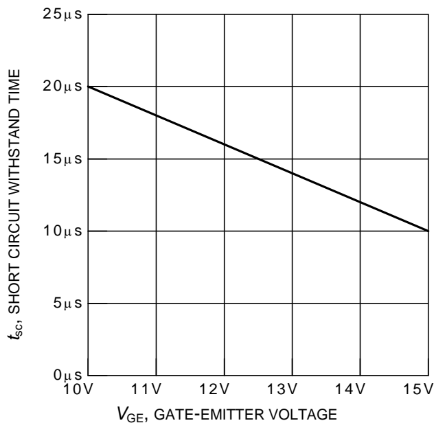
Figure 19. Short circuit withstand time as a function of gate-emitter voltage ( V_{CE} = 600V , start at T_i = 25^\circ C )
