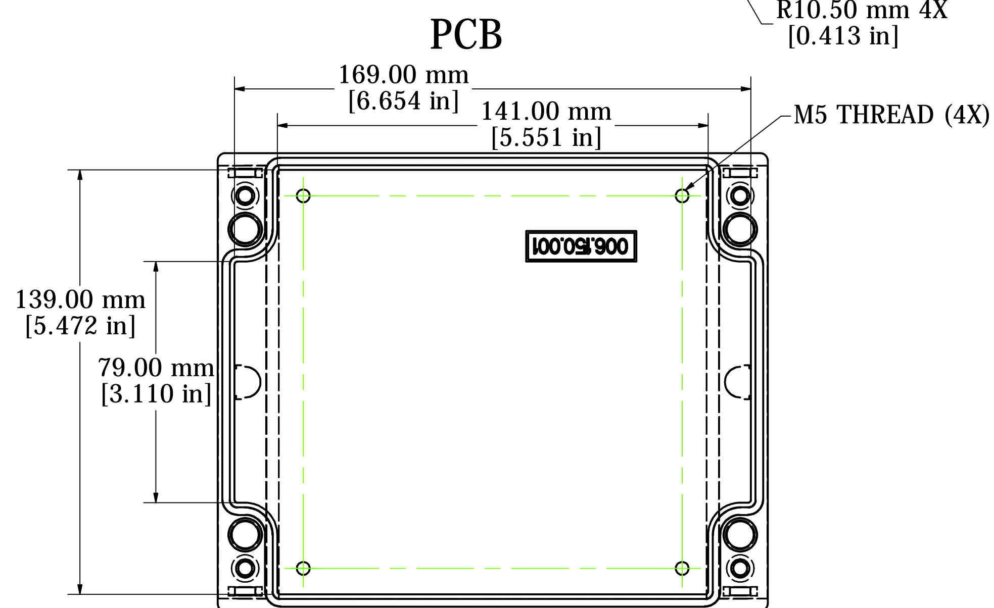
LID - INSIDE VIEW
