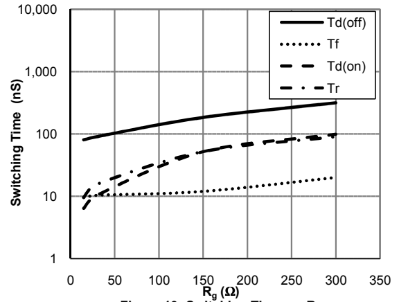
Figure 13: Switching Time vs. R_g ( T_j=150^\circ\text{C}, V_{GE}=15\text{V}, V_{CE}=400\text{V}, I_c=10\text{A} )
