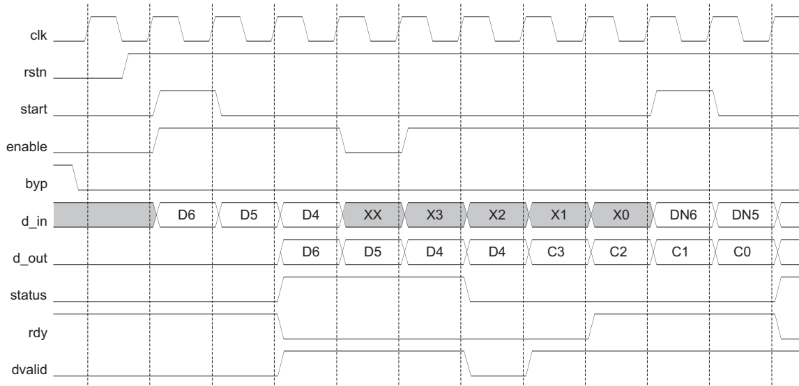
Figure 4. Timing of an RS (7,3) Single Pipelined Encoder with enable De-asserted
