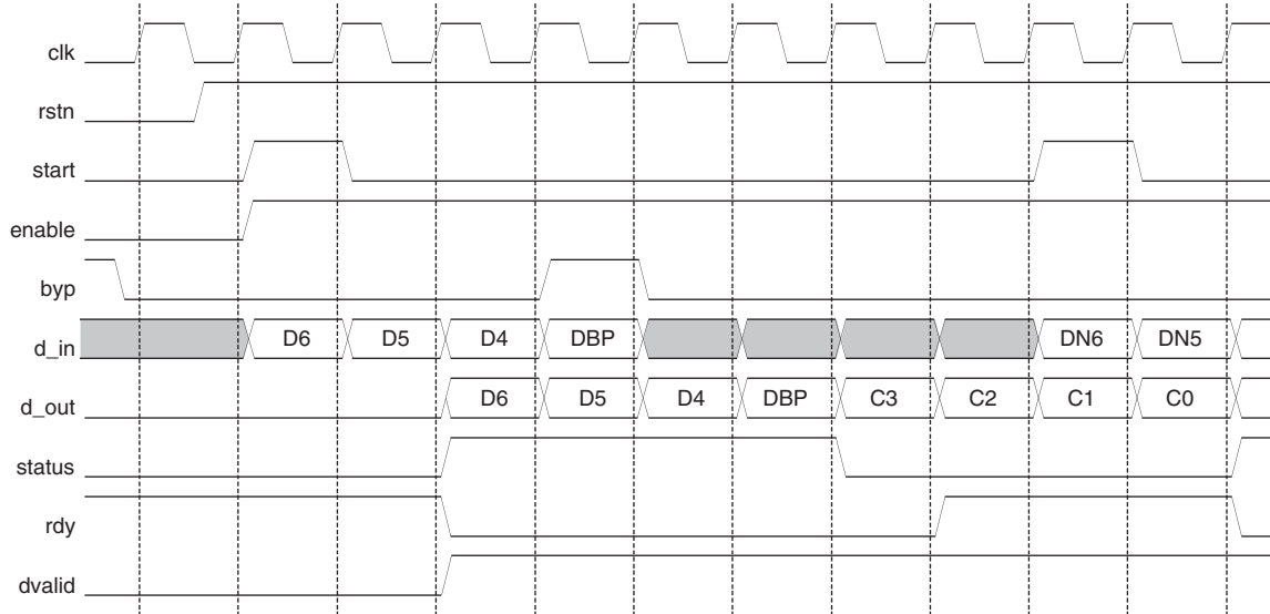
Figure 3. Timing of an RS (7,3) Single Pipelined Encoder with byp Asserted
