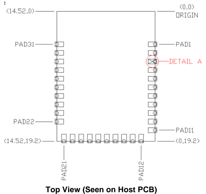
Figure 6. Solder Pad Reference Location
