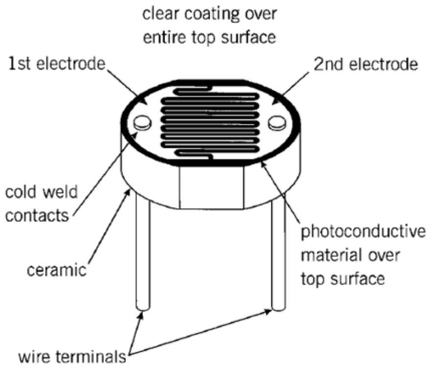
Figure 3 Typical Construction of a Plastic Coated Photocell
