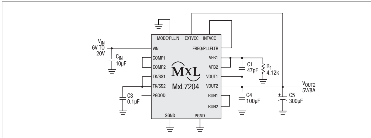
Figure 33: Output Paralleled for 5V at 8A Design
