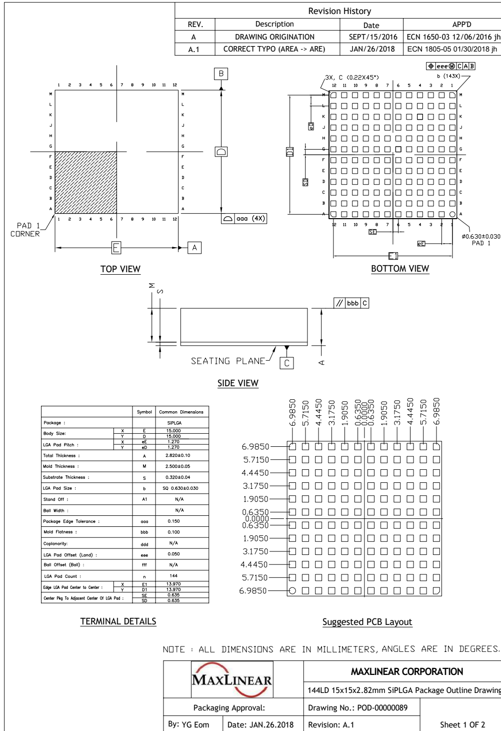
Figure 34: Mechanical Dimensions
