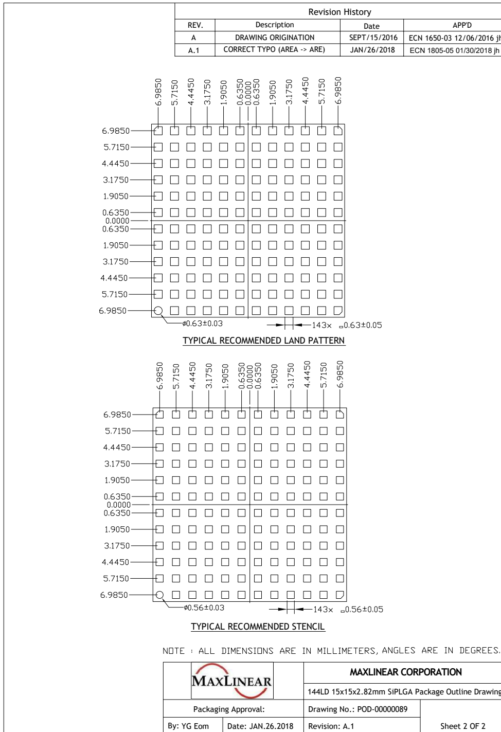
Figure 35: Recommended Land Pattern and Stencil
