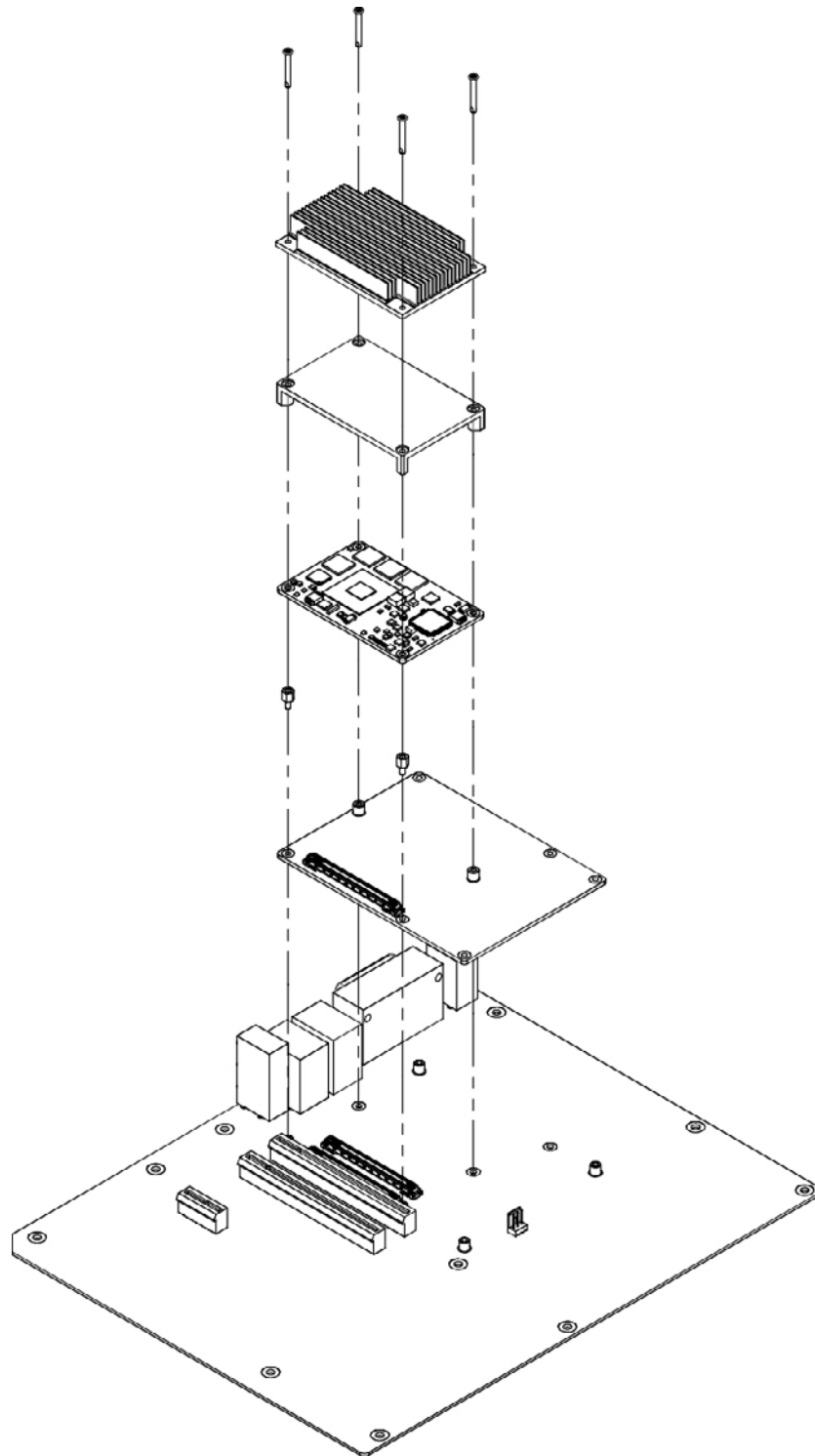
Figure 2.5 Assembly Drawing
