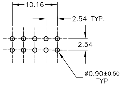
RECOMMENDED P.C.B. LAYOU
