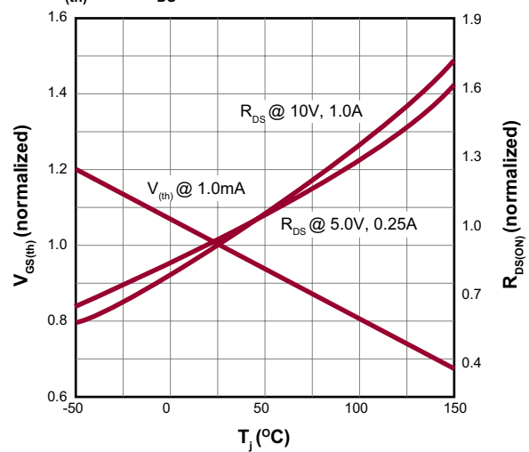
V_{GS(th)} and R_{DS} Variation with Temperature
