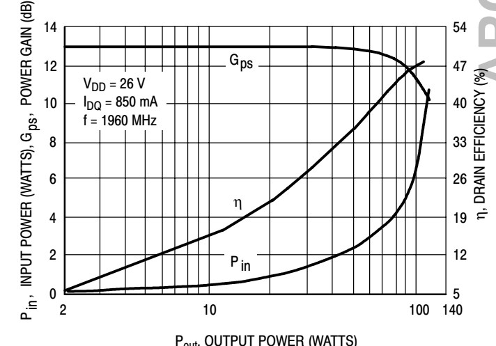
Figure 8. CW Performance
