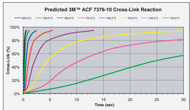
Figure 2. Graph of predicted cross-link reaction compared with bonding temperature and time.
