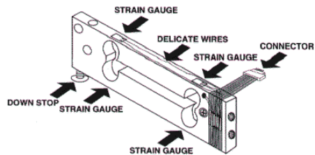
Strain gauge load cell diagram from Scalenet.com
