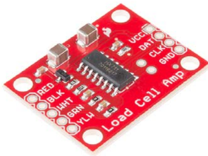
SparkFun's HX711 Amplifier breakout board
