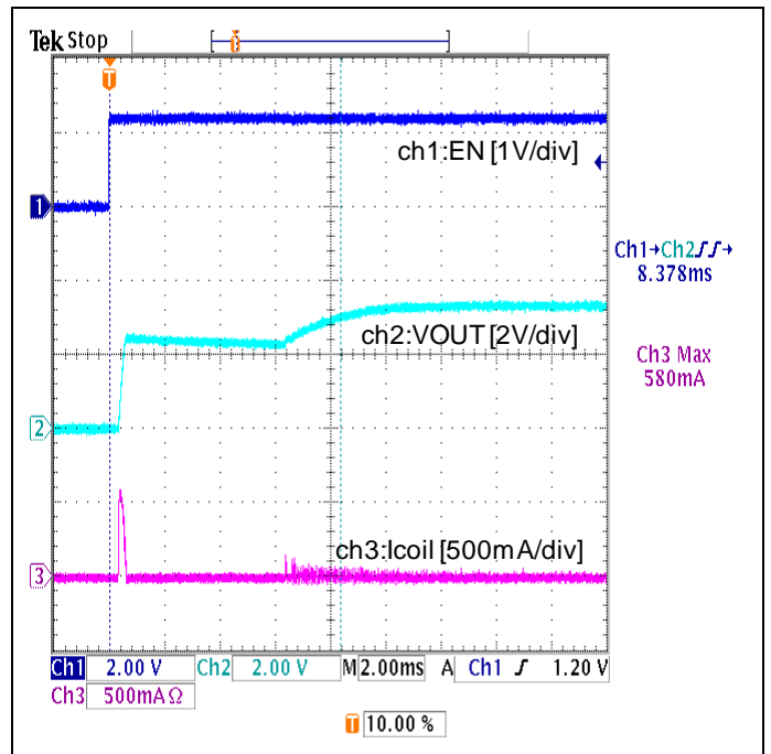
Figure 24. Start-up Waveform ( V_{IN}=2.4V , 3.3K\Omega resistive load, MODE=H:Auto-PFM/PWM)
