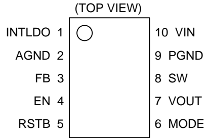
Figure 3. Pin Configuration
