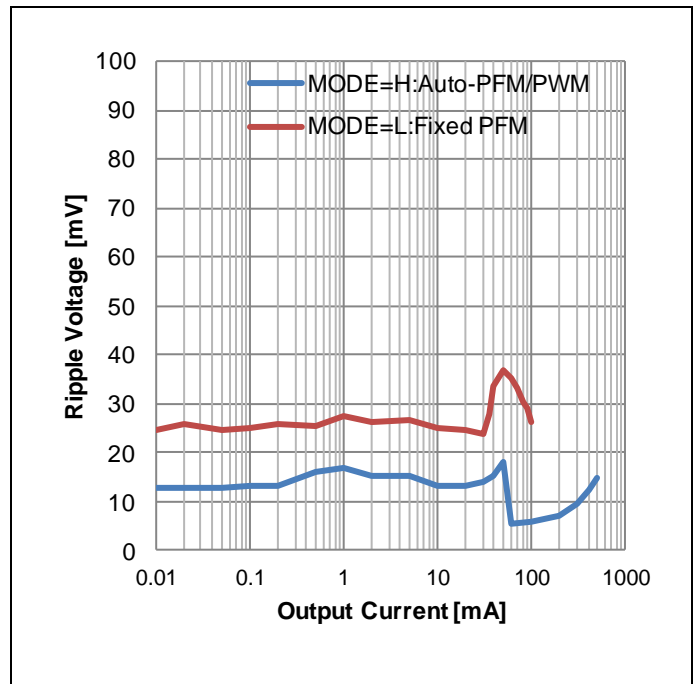
Figure 16. Ripple Voltage vs Output Current ("Ripple", VIN=2.4V)
