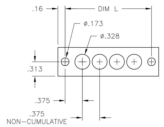
MOUNTING PANEL LAYOUT
