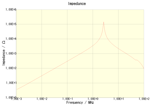
CLF7045T-471M-CA
