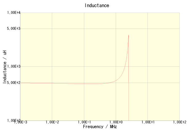
CLF7045T-471M-CA
