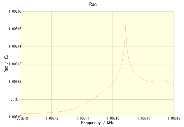
CLF7045T-471M-CA
