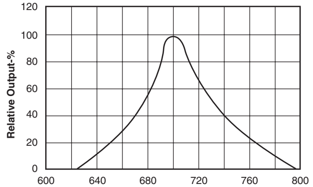
Fig. 2 Spectral Response
