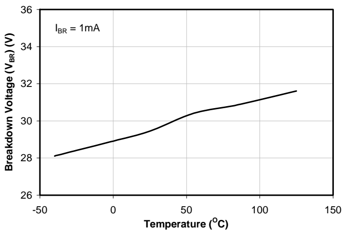
Typical Breakdown Voltage v Temperature
