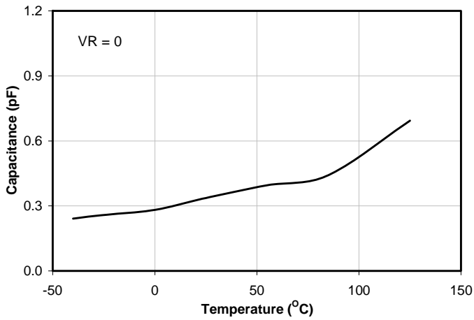
Typical Junction Capacitance v Temperature
