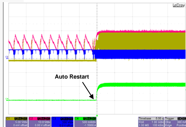
Figure 22. V_{IN} = 90 V_{AC} / 60 \text{ Hz} , [LED Restore]
