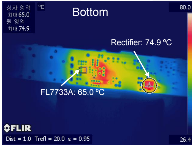
Figure 41. V_{IN} = 90 V_{AC} / 60 Hz
