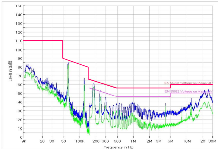
Figure 43. V_{IN} [110 V AC , Neutral]
