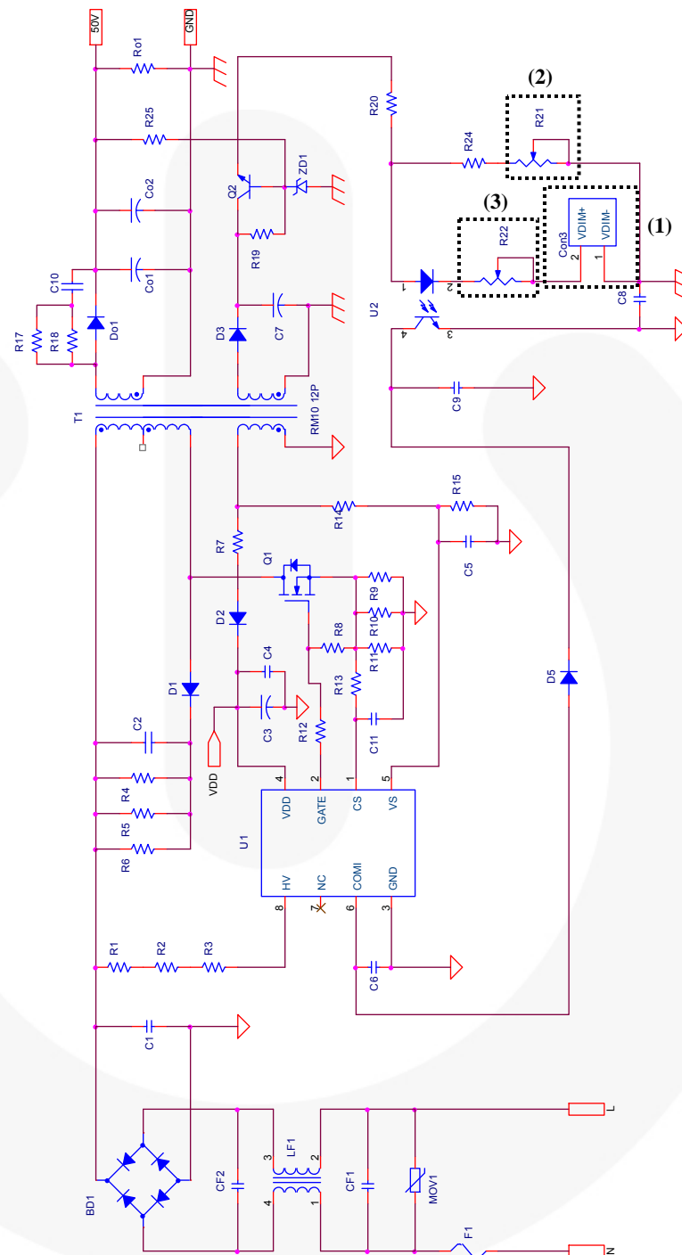
Figure 7. Schematic
