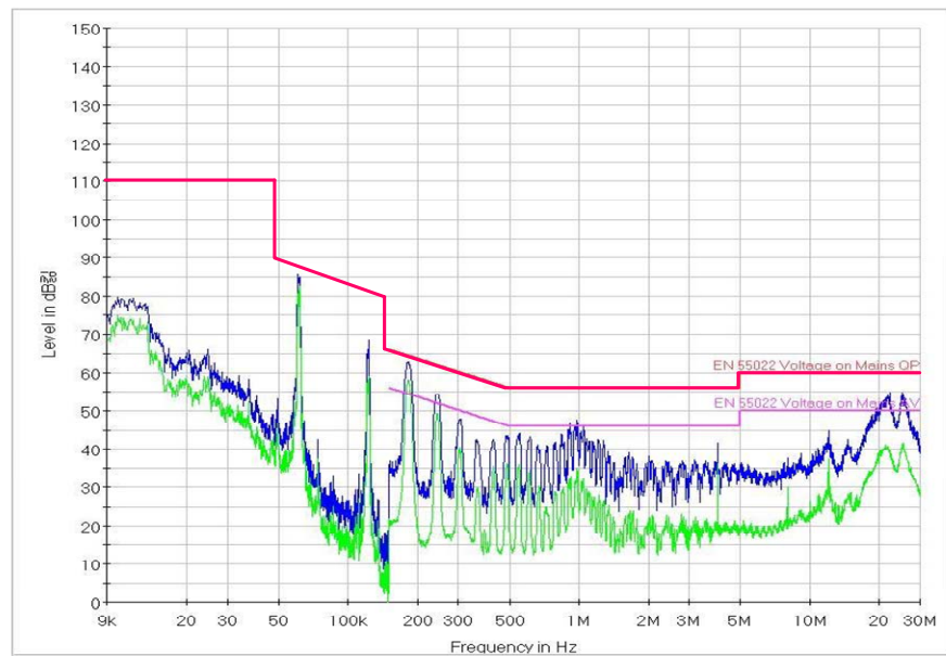
Figure 44. V_{IN} [220 V AC , Live]
