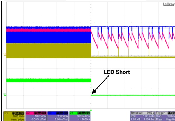
Figure 23. V_{IN} = 300 V_{AC} / 50 \text{ Hz} , [LED Short]
