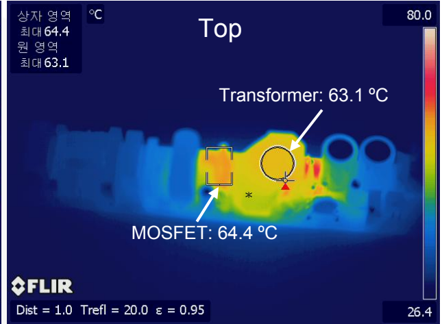
Figure 40. V_{IN} = 300 V_{AC} / 50 Hz
