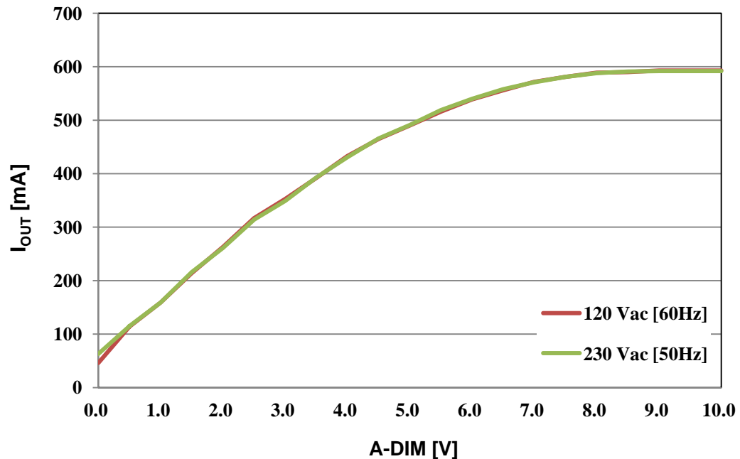
Figure 29. Analog Dimming
