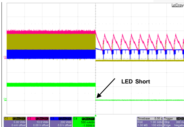
Figure 21. V_{IN} = 90 V_{AC} / 60 \text{ Hz} , [LED Short]
