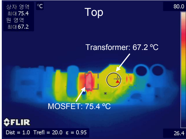
Figure 39. V_{IN} = 90 V_{AC} / 60 Hz
