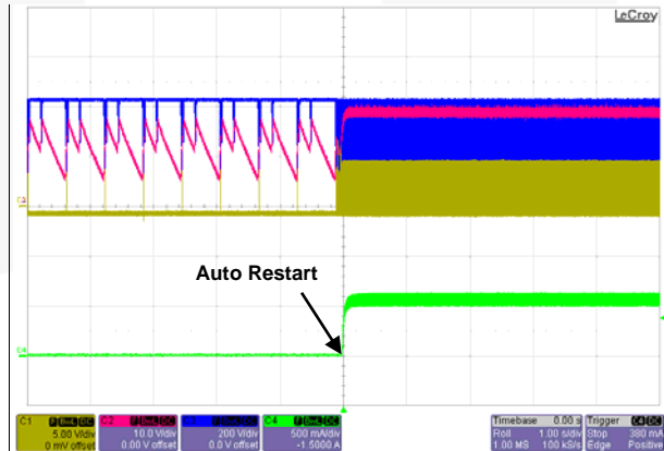
Figure 24. V_{IN} = 300 V_{AC} / 50 \text{ Hz} , [LED Restore]
