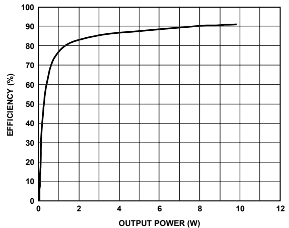
Figure 28. Efficiency vs. Output Power, 12 V, 8 \Omega
