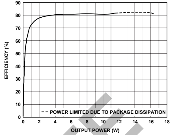
Figure 26. Efficiency vs. Output Power, 12 V, 4 \Omega
