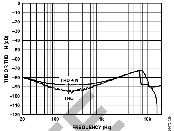
Figure 20. THD or THD + N vs. Frequency @ 1 W, 4 Ω, PVDD = 12 V, PGA = 0 dB
