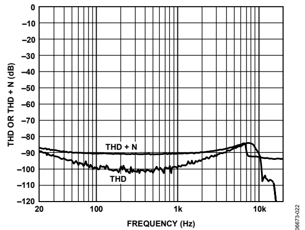
Figure 22. THD or THD + N vs. Frequency @ 1 W, 8 Ω, PVDD = 12 V, PGA = 0 dB
