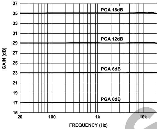
Figure 24. Gain vs. Frequency @ 1 W, 6 \Omega , PVDD = 12 V, 6 \Omega
