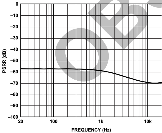
Figure 25. PSRR vs. Frequency, No Input Signal Ripple = 1.2 V p-p, PVDD = 12 V, 6 \Omega
