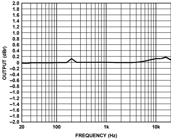
Figure 23. Frequency Response @ 1 W, 6 \Omega , PVDD = 12 V, PGA = 0 dB
